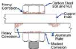
Effects of Galvanic Corrosion
